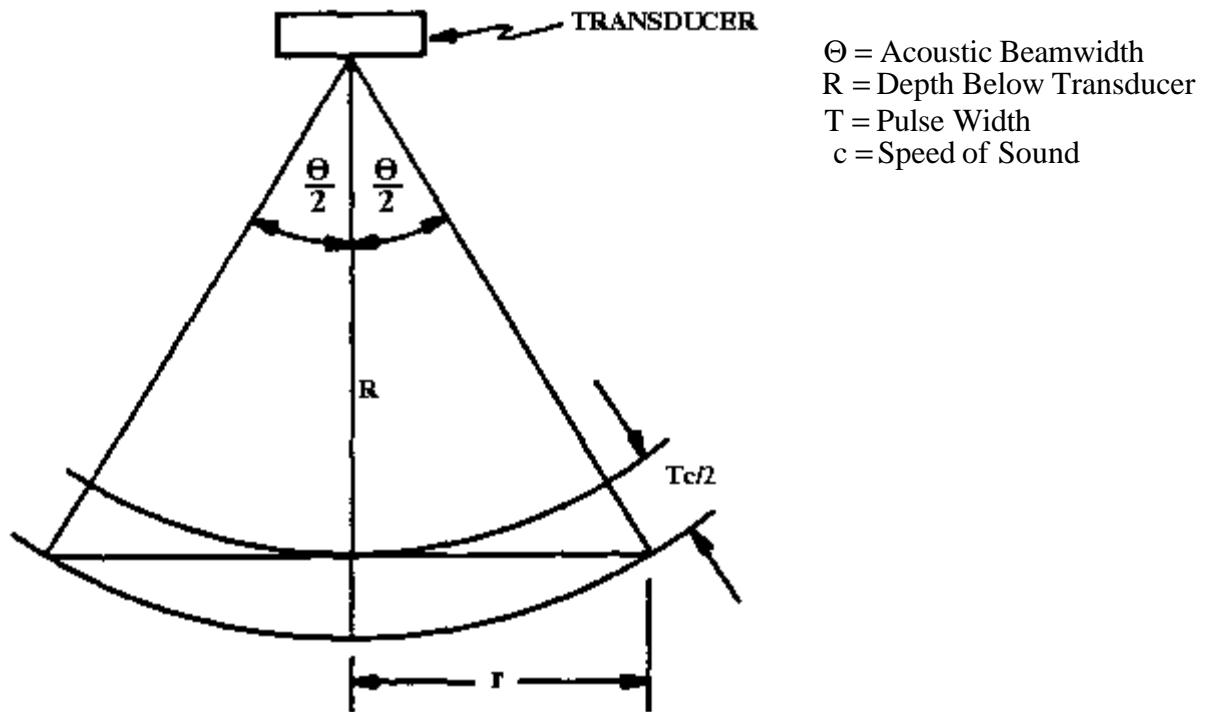
Figure 2 Function of the transmitted beamwidth, depth, and pulse duration
