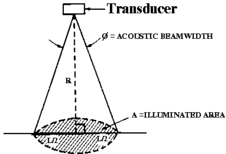
Figure 1 Area illuminated by a conical beam
