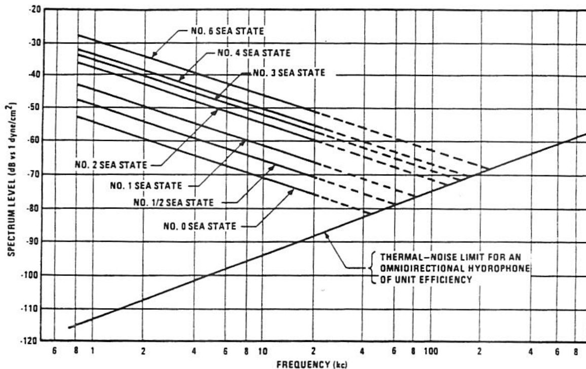
Figure 3. Deep Water Ambient Noise Levels
